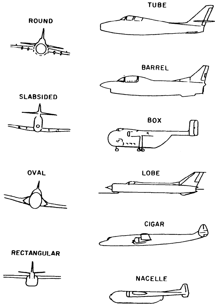
Figure 32.—Fuselage types.
