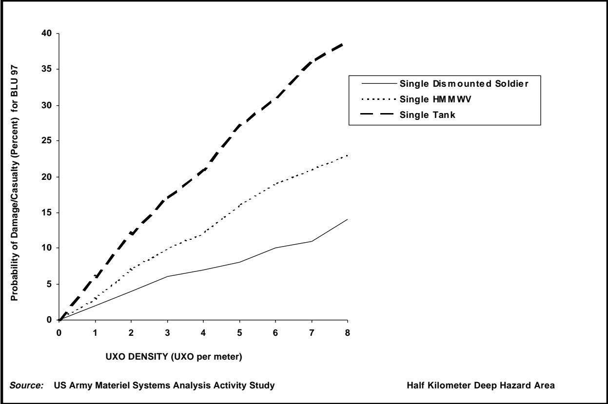
Figure I-4. UXO Expected Damage/Casualties Versus BLU 97 UXO Hazard Area Density
