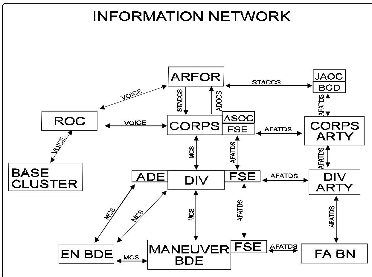
Figure III-1. Theater Army Information Network
