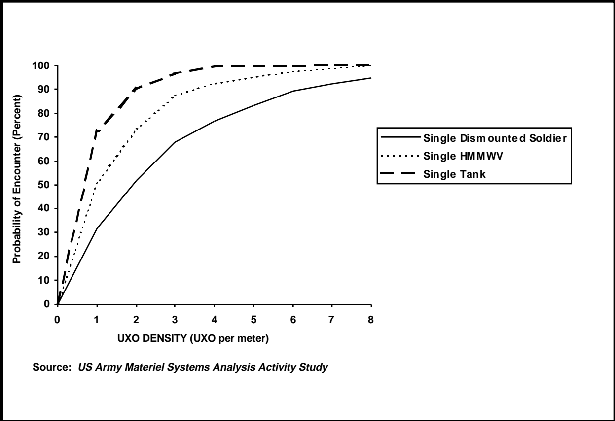
Figure I-2. Vehicle Submunition Encounter Probability Versus UXO Density
