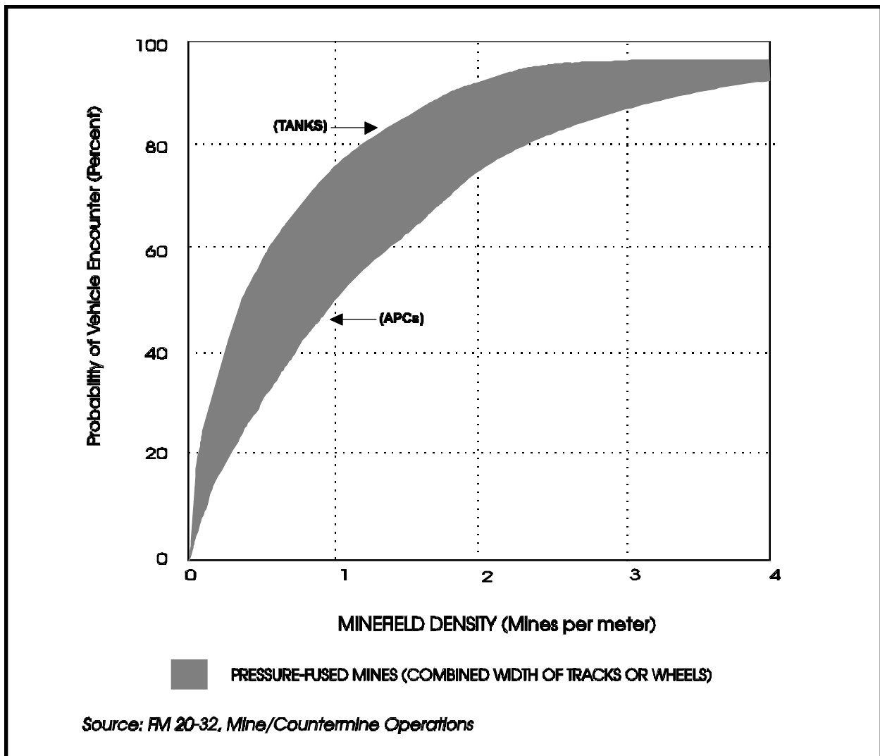
Figure I-1. Vehicle Mine Encounter Probability Versus Minefield Density
