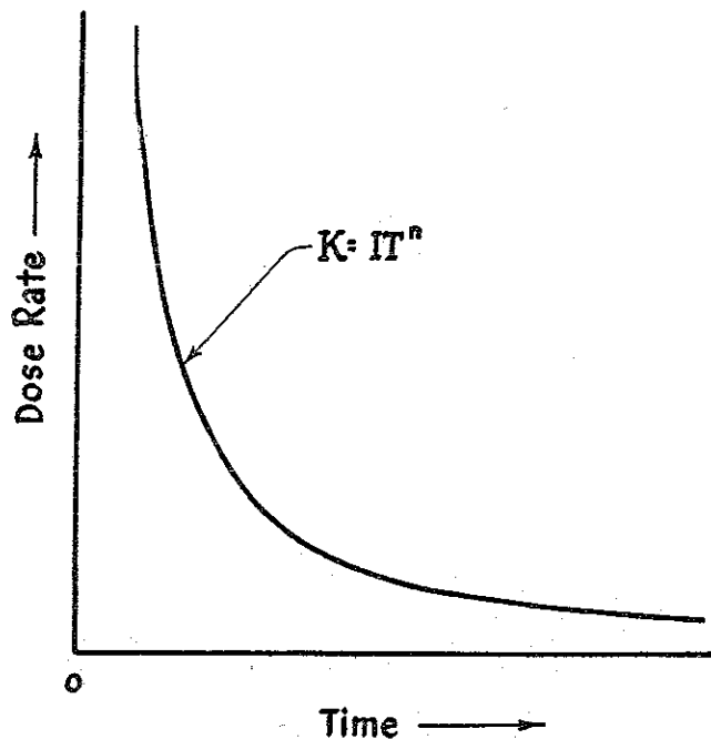
Figure 6—Multiple Decay.
